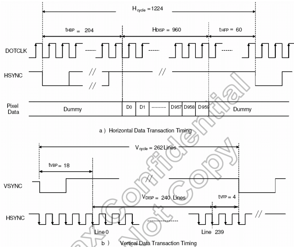
Data Transaction Timing in Serial RGB (8 bit) Interface (SYNC Mode)
